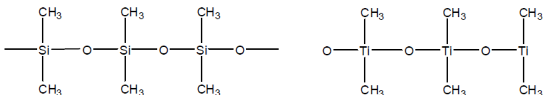
Polydimethylsiloxane
